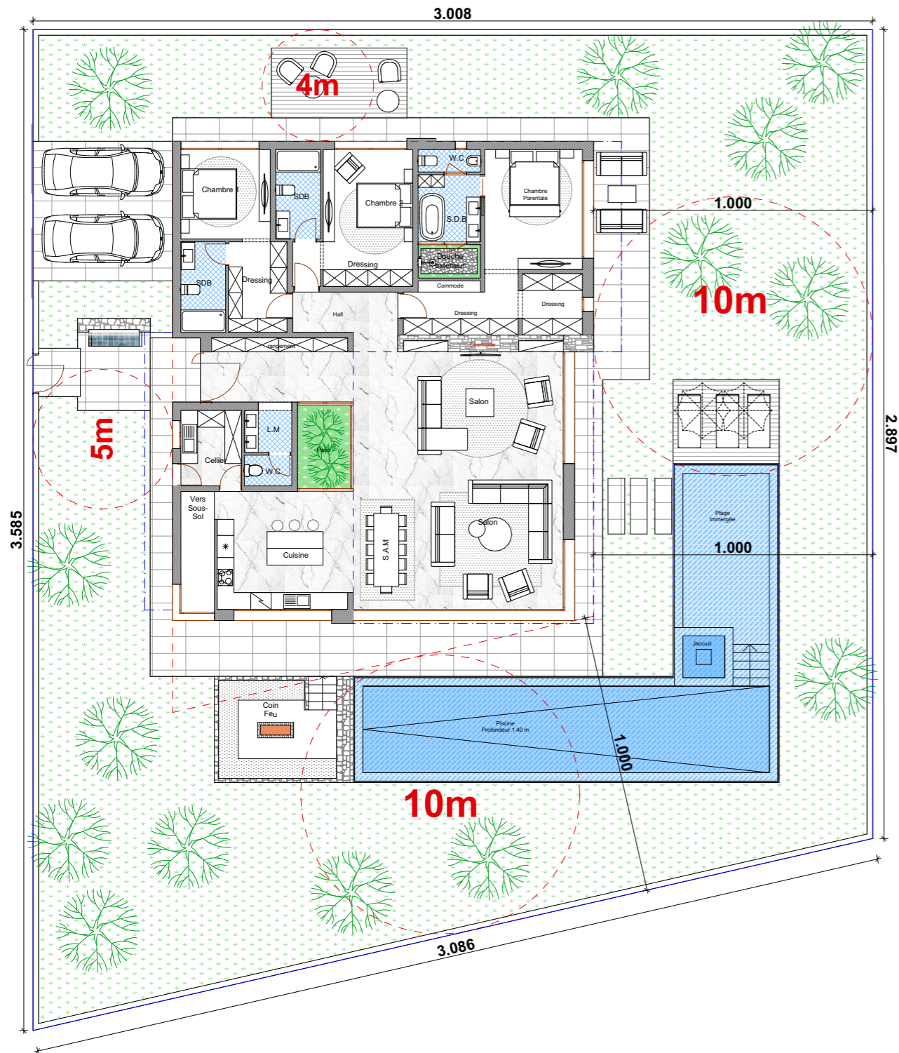
Plan RDC Surface couverte = 265 m 2
